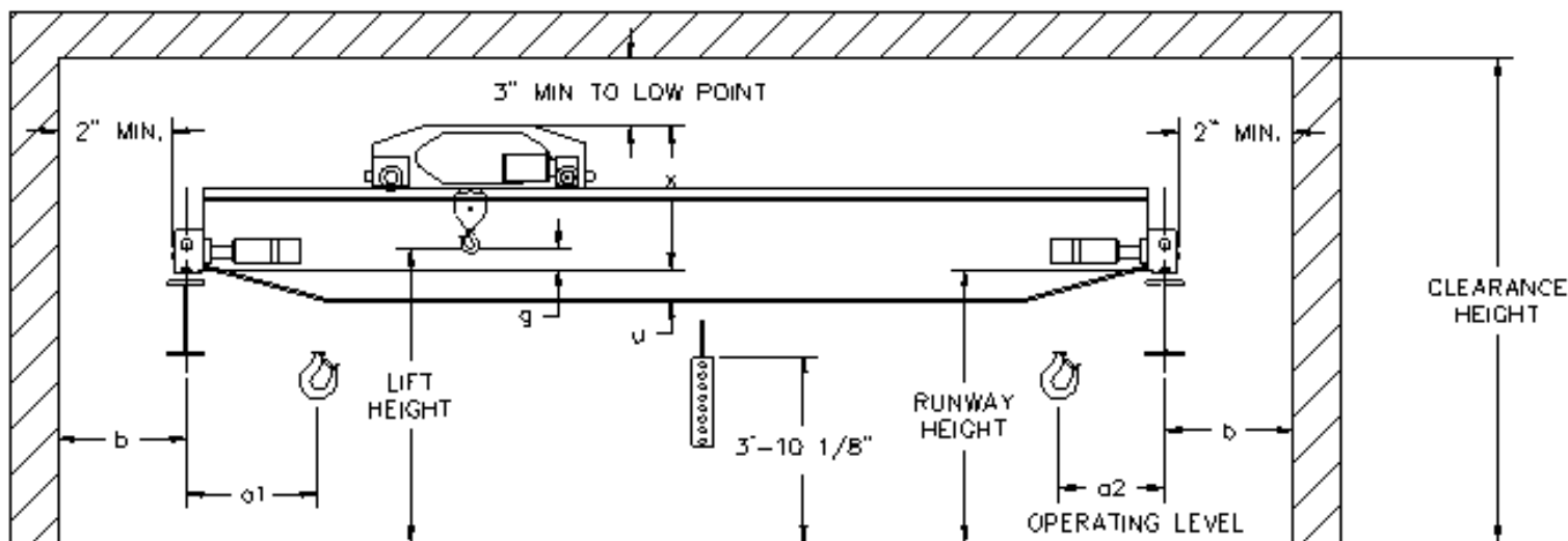
TOP RUNNING DOUBLE GIRDER CRANE
