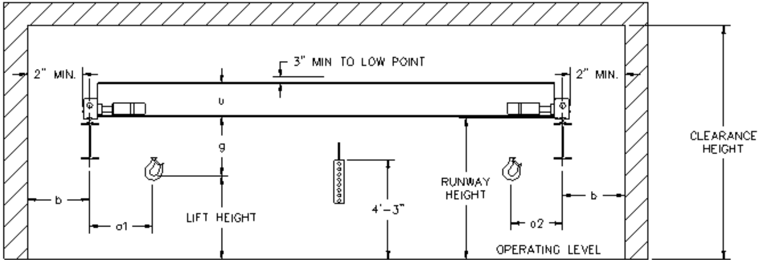
TOP RUNNING SINGLE GIRDER CRANE
